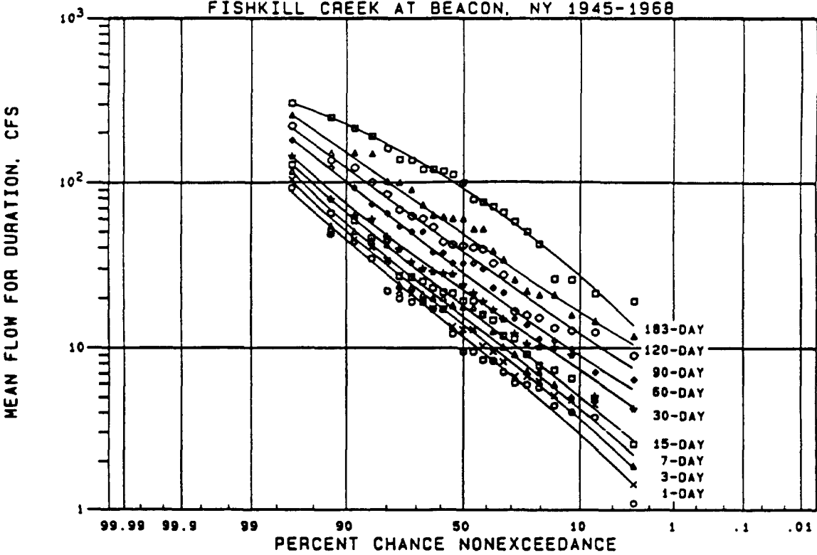
Figure 4-1. Low-Flow Frequency Curves.
